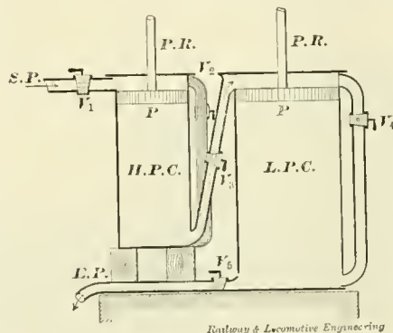
CYLINDERS OF FIRST COMPOUND ENGINE.
